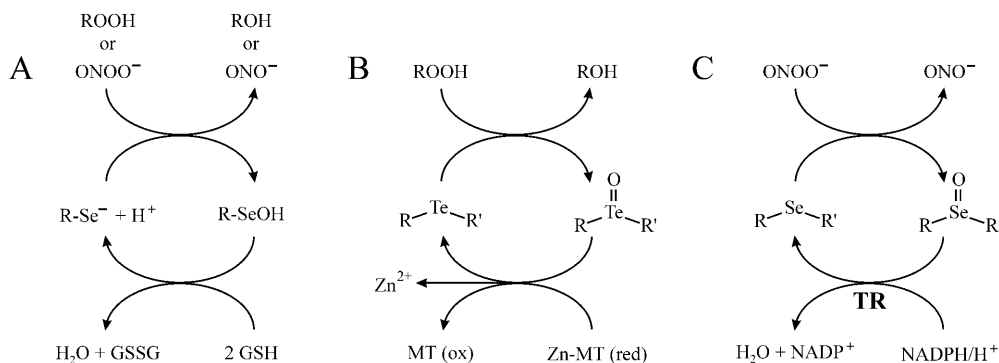
FIGURE 2 Proposed catalytic mechanisms for the reduction of hydroperoxides and peroxy-nitrite in the presence of seleno- and tellurocompounds. (A) The selenocysteine at the active site of GPx is oxidized to the corresponding selenenic acid by hydroperoxides or peroxy-nitrite, which in turn are reduced to the corresponding alcohol and nitrite, respectively. The reduced form of the enzyme is restored at the expense of GSH (5,6,37). (B) Several low-molecular-weight organoselenium and -tellurium compounds mimic the GPx reaction. The transiently formed respective selenoxide or telluroxide may be reduced by thiols other than glutathione including zinc-metallothionein (MT), which upon oxidation releases Zn^{2+} (42). (C) Mammalian thioredoxin reductase (TR) is a selenoenzyme and may reduce the oxidized forms of certain selenocompounds that are formed after interaction with peroxy-nitrite, such as the ebselen selenoxide, at the expense of NADPH (47).
